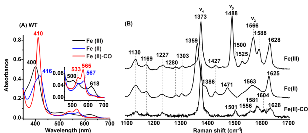
Figure 2. UV-vis (A) and high-frequency RR (B) spectra of WT hPGRMC1. The UV and RR spectra were obtained with \sim 5 and 80 \mu\text{M} protein, respectively, in 100 mM pH 7.4 potassium phosphate buffer.
