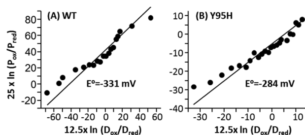
Figure 1. Linear Nernst plots based on one-electron reduction of WT (A) and Y95H mutant (B) of hPGRMC1 and two-electron reduction of a dye, safranin T. P_{ox}/P_{red} and D_{ox}/D_{red} stand for the ratio of oxidized protein vs reduced protein and the ratio of oxidized dye vs reduced dye, respectively. The solid lines are the best fit lines with the slopes fixed to be 1. The redox potentials of the WT and Y95H mutant of hPGRMC are estimated based on the intercepts of the lines to be ~−331 and −284 mV, respectively, with the assumption that E^{\circ} (safranin T) = −289 mV (vs SHE).
