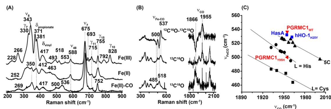
Figure 3. Low-frequency RR spectra (A) and CO isotope-sensitive \nu_{\text{Fe-CO}}/\nu_{\text{C-O}} modes of WT hPGRMC1 (B). \nu_{\text{Fe-CO}} vs \nu_{\text{C-O}} inverse correlation plot (C). In (C), the data points associated with P450s (L = Cys), myoglobin variants (L-His), and 5C heme are taken from the literature 27,42,44,62,63 and are presented by black squares, circles, and triangles, respectively; those associated with PGRMC1, HasA, 44 and H25Y mutant of hHO-1 27 are as indicated. The data were obtained with \sim 80 \mu\text{M} protein in 100 mM pH 7.4 potassium phosphate buffer.
