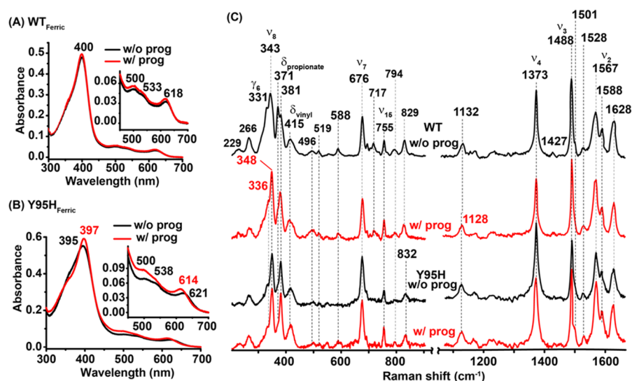
Figure 5. UV-vis (A, B) and RR (C) spectra of the WT and Y95H mutant of ferric hPGRMC1 with (red) and without (black) progesterone. The concentrations of protein/progesterone are \sim 5/50 and 80/500 \mu\text{M} (in 100 mM pH 7.4 potassium phosphate buffer) for the UV-vis and RR measurements, respectively.
