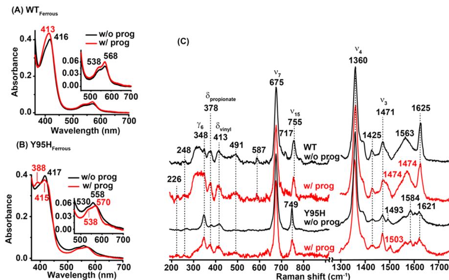
Figure 6. UV-vis (A, B) and RR (C) spectra of the WT and Y95H mutant of deoxy ferrous hPGRMC1 with (red) and without (black) progesterone. The concentrations of protein/progesterone are \sim 5/50 and 80/500 \mu\text{M} (in 100 mM pH 7.4 potassium phosphate buffer) for the UV-vis and RR measurements, respectively.
